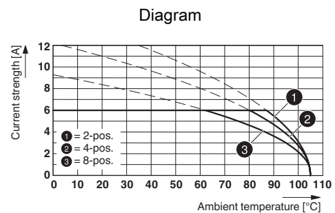
Type: PTCM 0,5/...-PL-2,5 WH with PTSM 0,5/...-HH(0)-2,5-SMD WH R...
